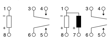
<2 Form A> Single side stable (Deenergized condition) 2 coil latching (Reset condition)
